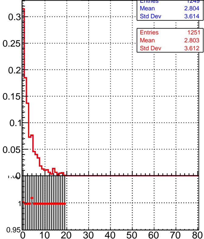
■ DQM_TT_mkFit-DQM_pless_orig ● DQM_TT_mkFit-DQM_pless_modi
