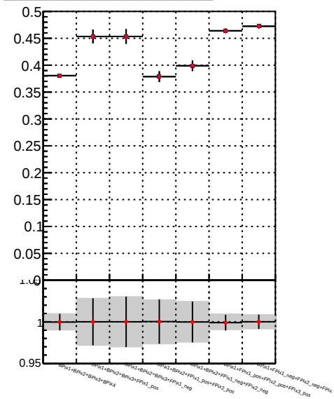
Fake rate vs. DQM TT_mkFit-DQM_pless_orig DQM TT_mkFit-DQM_pless_modi
