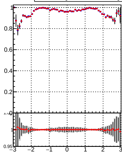
—■— DQM_TT_mkFit-DQM_pless_orig —●— DQM_TT_mkFit-DQM_pless_modi
