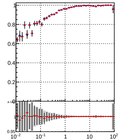
—•— DQM_TT_mkFit-DQM_pless_orig —•— DQM_TT_mkFit-DQM_pless_modi
