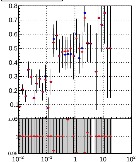
—•— DQM_TT_mkFit-DQM_pless_orig —•— DQM_TT_mkFit-DQM_pless_modi
