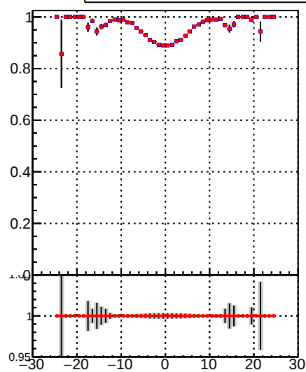
—•— DQM_TT_mkFit-DQM_pless_orig —•— DQM_TT_mkFit-DQM_pless_modi
