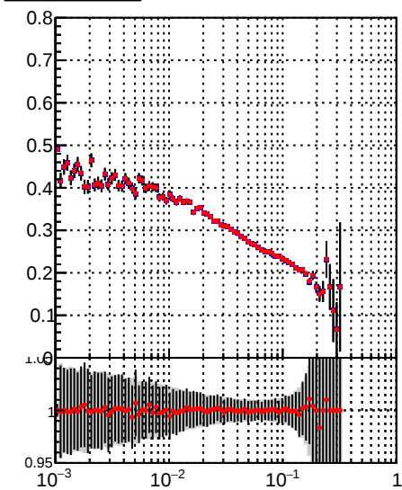
—•— DQM_TT_mkFit-DQM_pless_orig —•— DQM_TT_mkFit-DQM_pless_modi
