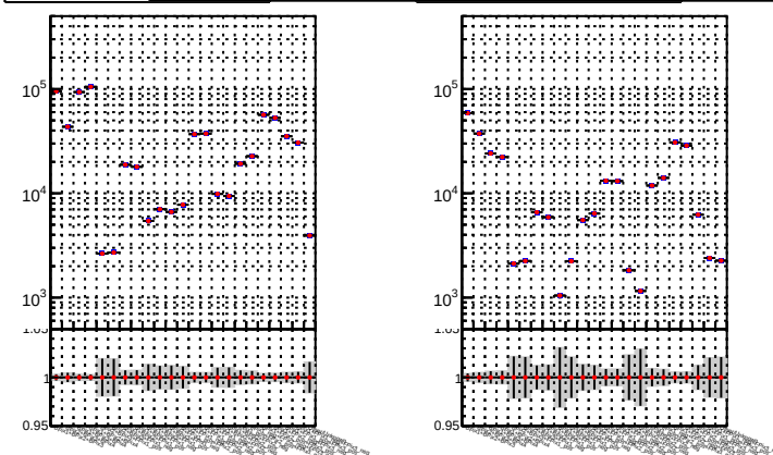
N of reco track vs. \chi^2
