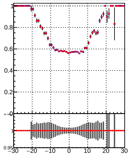
—•— DQM_TT_mkFit-DQM_pless_orig —•— DQM_TT_mkFit-DQM_pless_modi
