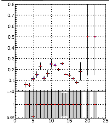
Efficiency vs hit Legend: DQM_TT_mkFit-DQM_pless_orig DQM_TT_mkFit-DQM_pless_modi
