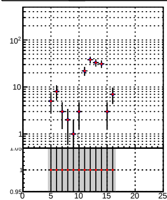
Legend: DQM_TT_mkFit-DQM_pless_orig (blue line with dots) DQM_TT_mkFit-DQM_pless_modi (red line with dots)
