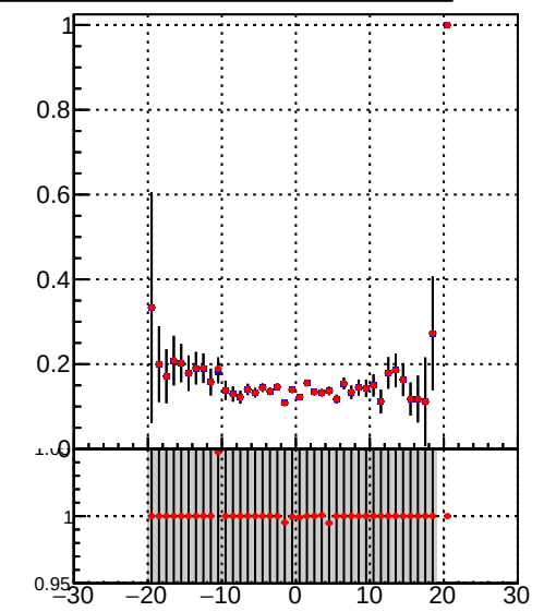
Efficiency vs. sim PV z Legend: DQM_TT_mkFit-DQM_pless_orig (blue line with error bars) DQM_TT_mkFit-DQM_pless_modi (red line with error bars)
