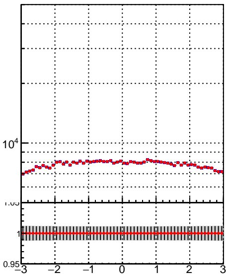
■ DQM_TT_mkFit-DQM_pless_orig ● DQM_TT_mkFit-DQM_pless_modi
