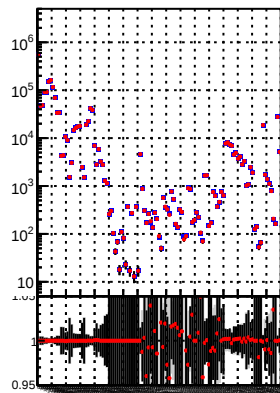
N of reco track vs. \chi^2
