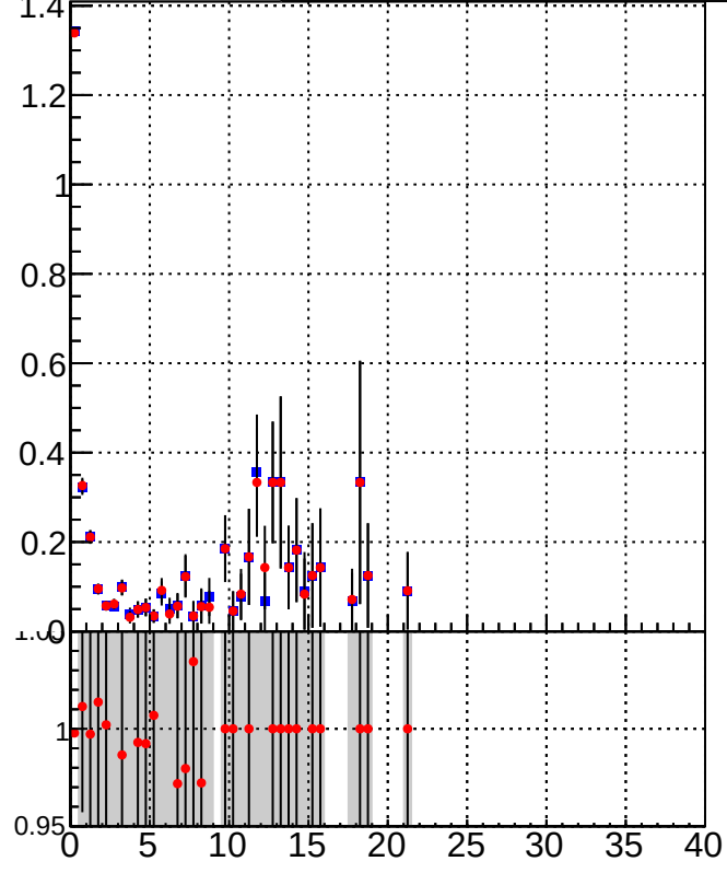
K_S^0 tracking fake rate vs p_T and \eta Legend: \blacksquare DQM_TT_mkFit-DQM_pless_orig \bullet DQM_TT_mkFit-DQM_pless_modi
