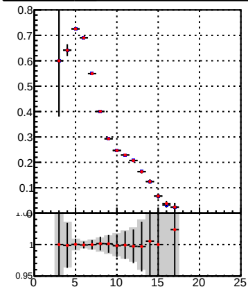
Legend: DQM_TT_mkFit-DQM_pless_orig (grey line), DQM_TT_mkFit-DQM_pless_modi (red line)
