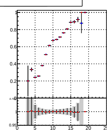
Legend: DQM_TT_mkFit-DQM_pless_orig (grey line), DQM_TT_mkFit-DQM_pless_modi (red line)
