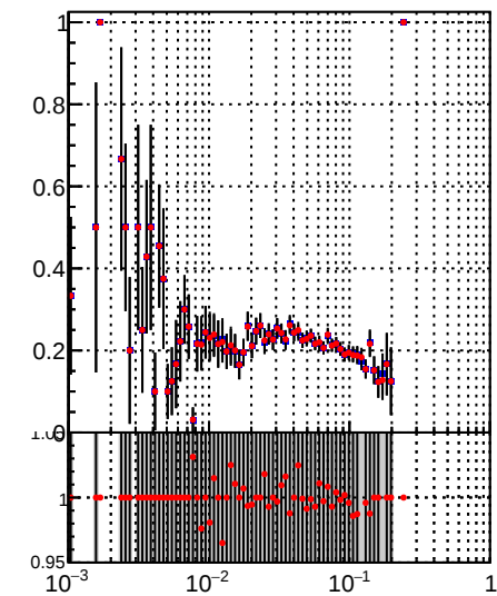
—•— DQM_TT_mkFit-DQM_pless_orig —•— DQM_TT_mkFit-DQM_pless_modi
