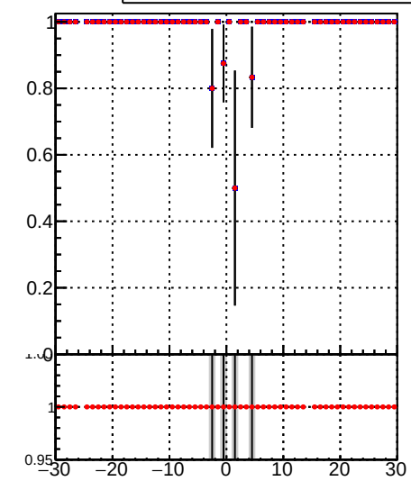
Fake rate vs vertpos Legend: DQM_TT_mkFit-DQM_pless_orig DQM_TT_mkFit-DQM_pless_modi
