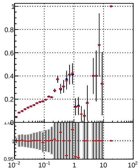
—•— DQM_TT_mkFit-DQM_pless_orig —•— DQM_TT_mkFit-DQM_pless_modi
