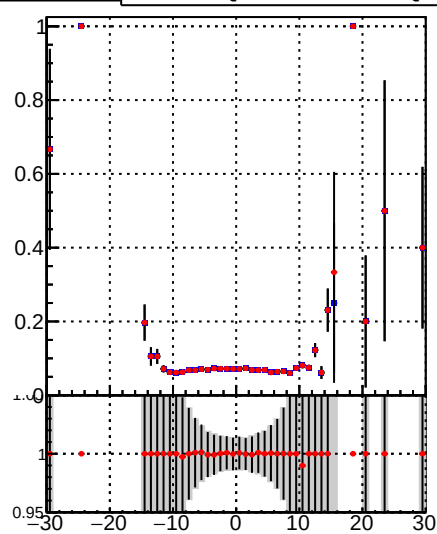
—•— DQM_TT_mkFit-DQM_pless_orig —•— DQM_TT_mkFit-DQM_pless_modi
