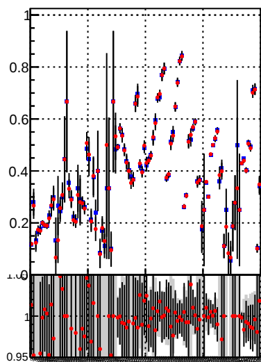
Fake rate vs. Legend for the bottom row of plots: —•— DQM TT mkFit-DQM_pless_orig —•— DQM TT mkFit-DQM_pless_modi
