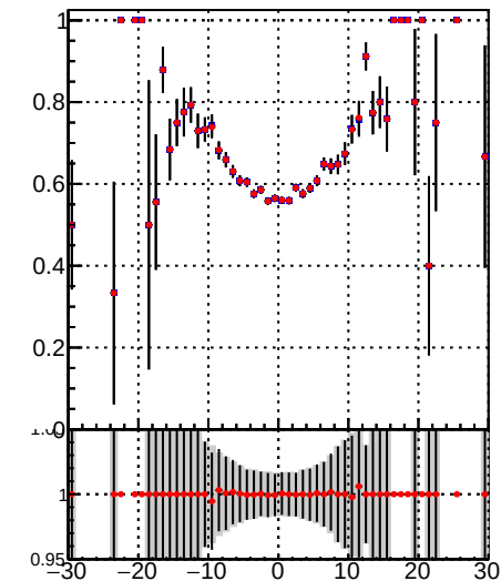
—•— DQM_TT_mkFit-DQM_pless_orig —•— DQM_TT_mkFit-DQM_pless_modi
