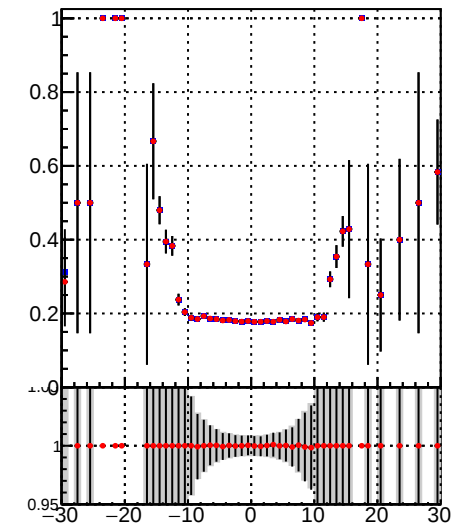
—•— DQM_TT_mkFit-DQM_pless_orig —•— DQM_TT_mkFit-DQM_pless_modi
