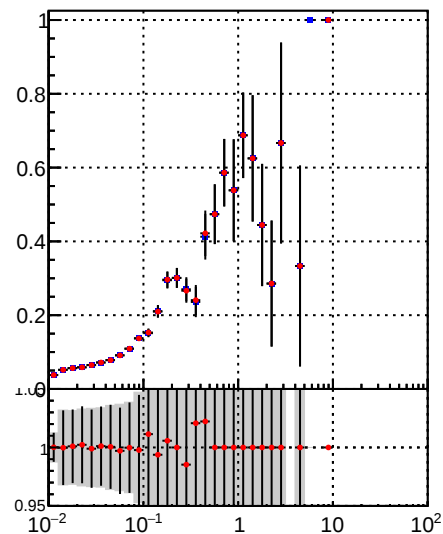
—●— DQM_TT_mkFit-DQM_pless_orig —●— DQM_TT_mkFit-DQM_pless_modi
