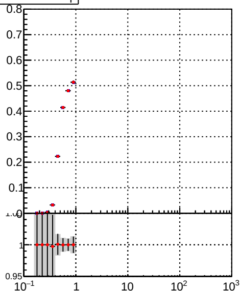
DQM_TT_mkFit-DQM_lowptq_orig DQM_TT_mkFit-DQM_lowptq_mod
