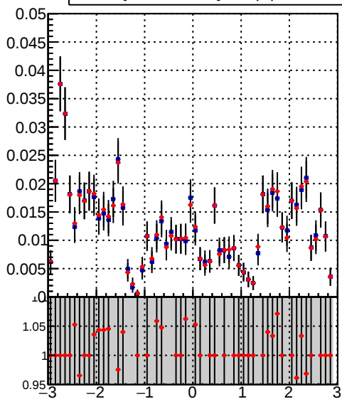
Legend: DQM_TT_mkFit-DQM_lowptq_orig DQM_TT_mkFit-DQM_lowptq_mod
