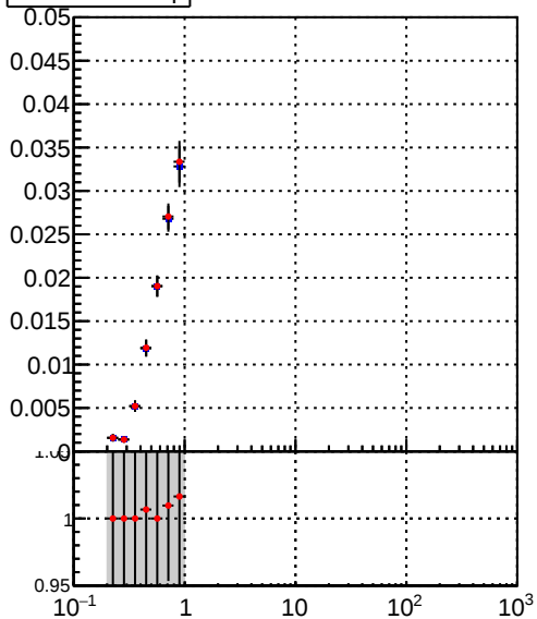
Legend: DQM_TT_mkFit-DQM_lowptq_orig DQM_TT_mkFit-DQM_lowptq_mod
