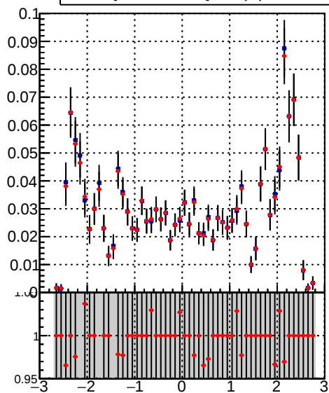
—•— DQM_TT_mkFit-DQM_lowptq_orig —•— DQM_TT_mkFit-DQM_lowptq_mod
