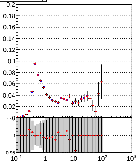
—•— DQM_TT_mkFit-DQM_lowptq_orig —•— DQM_TT_mkFit-DQM_lowptq_mod
