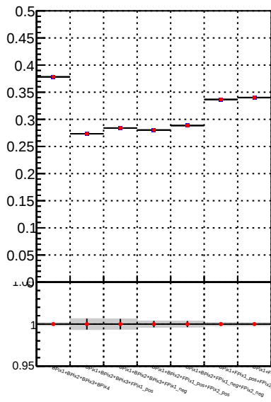
Fake rate vs. DQM_TT_mkFit-DQM_lowptq_orig DQM_TT_mkFit-DQM_lowptq_mod
