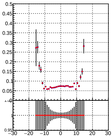
Fake rate vs d —•— DQM_TT_mkFit-DQM_lowptq_orig —•— DQM_TT_mkFit-DQM_lowptq_mod
