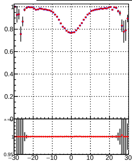
Legend: DQM_TT_mkFit-DQM_lowptq_orig (grey line with error bars) DQM_TT_mkFit-DQM_lowptq_mod (red line with error bars)
