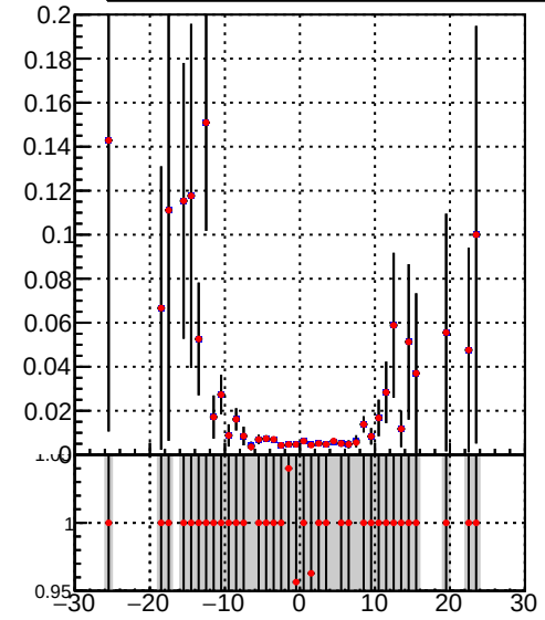
Efficiency vs vertpos Legend: DQM_TT_mkFit-DQM_lowptq_orig DQM_TT_mkFit-DQM_lowptq_mod
