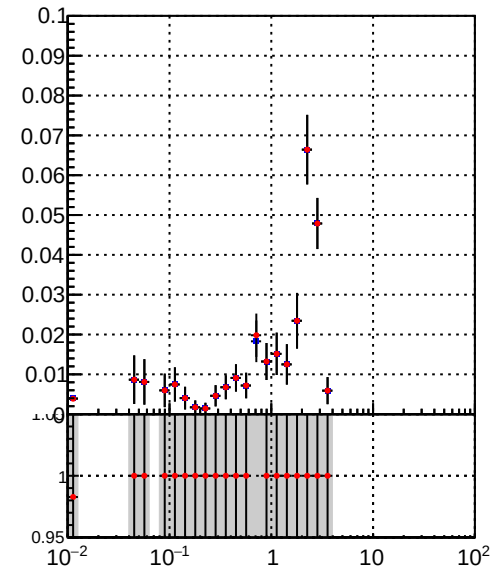
Efficiency vs vertpos Legend: DQM_TT_mkFit-DQM_lowptq_orig DQM_TT_mkFit-DQM_lowptq_mod
