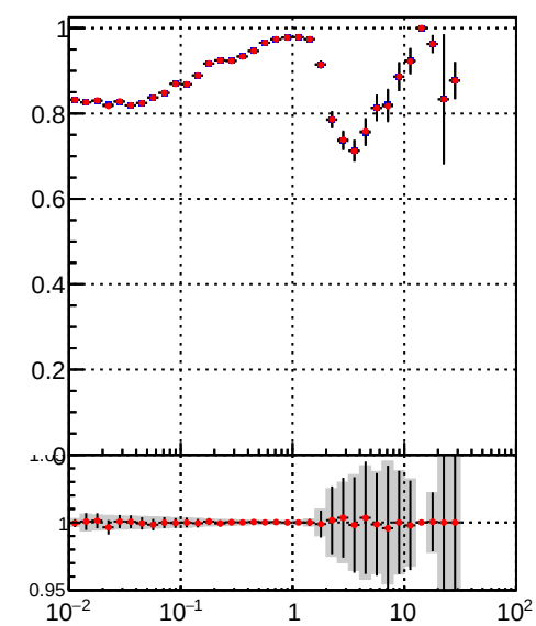
Efficiency vs vertpos Legend: DQM_TT_mkFit-DQM_lowptq_orig DQM_TT_mkFit-DQM_lowptq_mod
