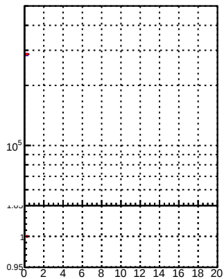
N of reco track vs. \chi^2 —•— DQM TT mkFit-DQM_lowtpq_orig —•— DQM TT mkFit-DQM_lowtpq_mod
