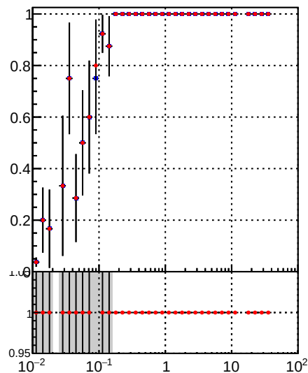
—•— DQM_TT_mkFit-DQM_lowptq_orig —•— DQM_TT_mkFit-DQM_lowptq_mod
