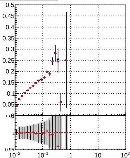
—•— DQM_TT_mkFit-DQM_lowptq_orig —•— DQM_TT_mkFit-DQM_lowptq_mod
