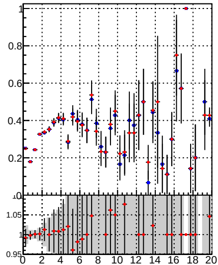
Fake rate vs. \text{mkFit-DQM\_lowptq\_orig} \text{mkFit-DQM\_lowptq\_mod}
