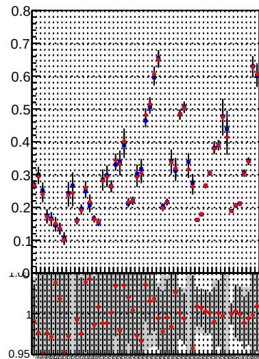
Fake rate vs. \text{mkFit-DQM\_lowptq\_orig} \text{mkFit-DQM\_lowptq\_mod}
