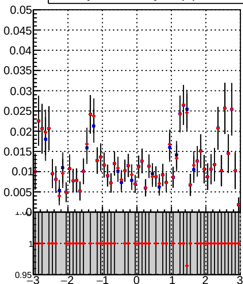
— DQM_TT_mkFit-DQM_lowptq_orig — DQM_TT_mkFit-DQM_lowptq_mod
