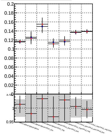
Fake rate vs. —●— DQM TT mkFit-DQM_lowptq_orig —●— DQM TT mkFit-DQM_lowptq_mod
