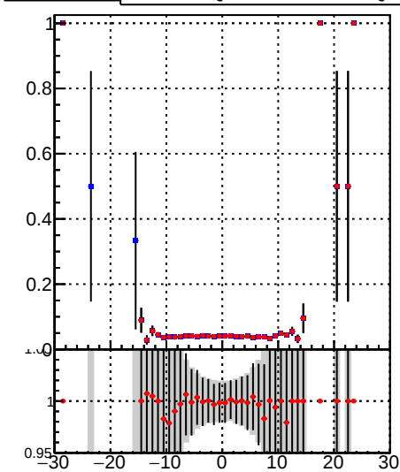
—•— DQM_TT_mkFit-DQM_lowptq_orig —•— DQM_TT_mkFit-DQM_lowptq_mod
