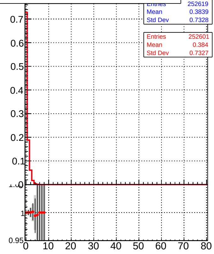
Legend: DQM_TT_mkFit-DQM_lowptq_orig (grey histogram) DQM_TT_mkFit-DQM_lowptq_mod (red line with points)
