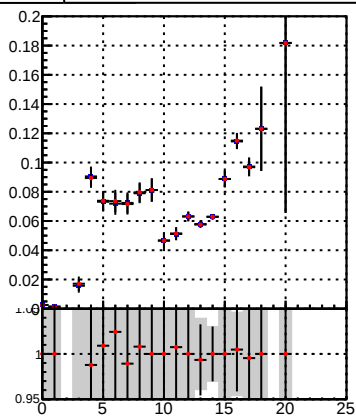
Efficienc — DQM_TT_mkFit-DQM_lowptq_mod
