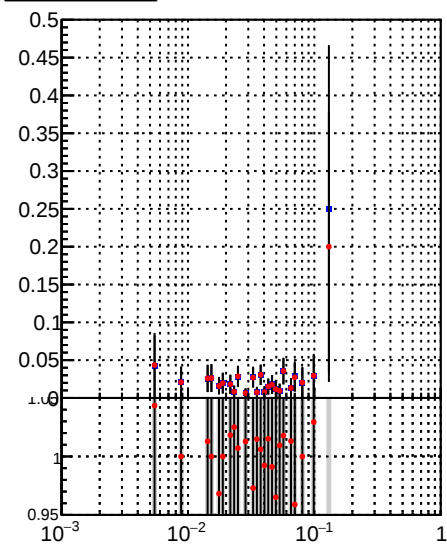
—•— DQM_TT_mkFit-DQM_lowptq_orig —•— DQM_TT_mkFit-DQM_lowptq_mod
