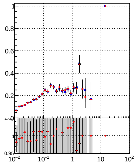
—●— DQM_TT_mkFit-DQM_lowptq_orig —●— DQM_TT_mkFit-DQM_lowptq_mod
