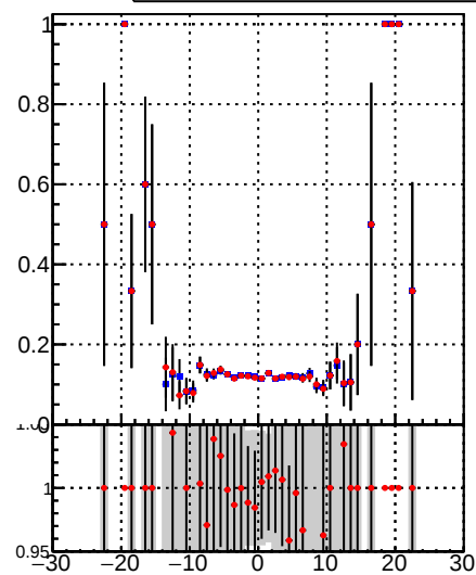
—●— DQM_TT_mkFit-DQM_lowptq_orig —●— DQM_TT_mkFit-DQM_lowptq_mod
