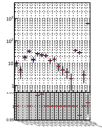
N of reco track vs. \chi^2 — mkFit-DQM_lowptq_orig — mkFit-DQM_lowptq_mod
