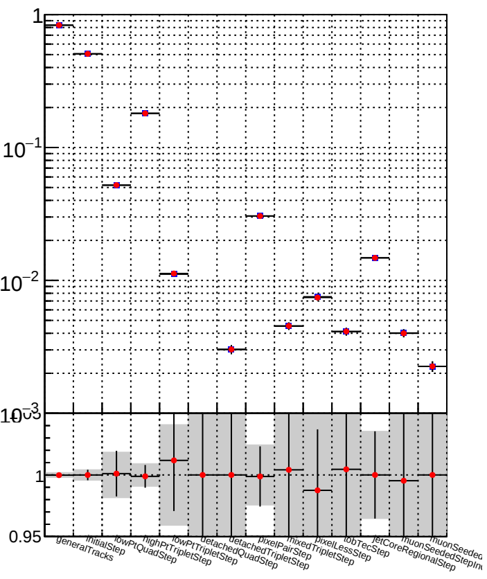
Duplicates rate vs collection Legend: ■ DQM_TT_mkFit-DQM_lowptq_orig ● DQM_TT_mkFit-DQM_lowptq_mod
