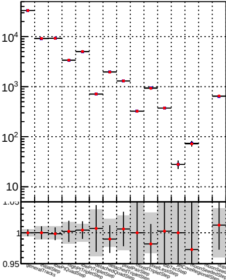
Number 1 DQM_TT__mkFit-DQM_lowptq_mod
