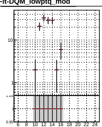
Legend: DQM_TT_mkFit-DQM_lowptq_orig (grey shaded area), DQM_TT_mkFit-DQM_lowptq_mod (red crosses with error bars)
