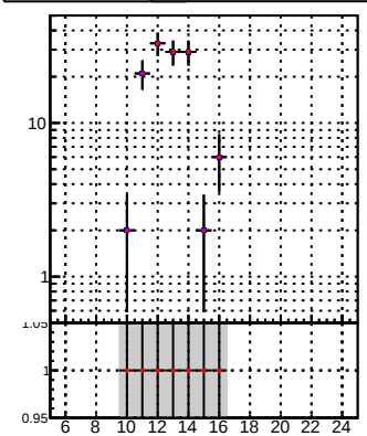
Legend: DQM_TT_mkFit-DQM_lowptq_orig (grey shaded area), DQM_TT_mkFit-DQM_lowptq_mod (red crosses with error bars)
