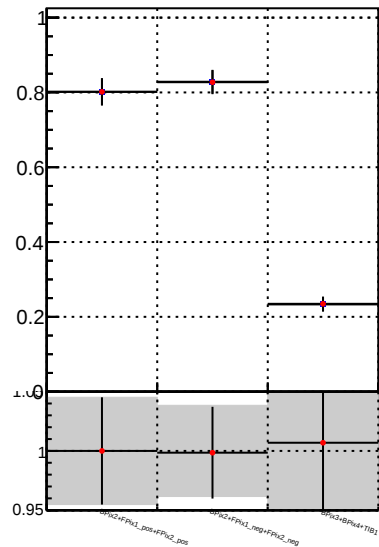
Fake rate vs. DQM_TT_mkFit-DQM_lowptq_orig DQM_TT_mkFit-DQM_lowptq_mod
