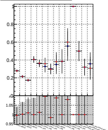
Fake rate vs. — DQM_TT_mkFit-DQM_lowptq_orig — DQM_TT_mkFit-DQM_lowptq_mod
