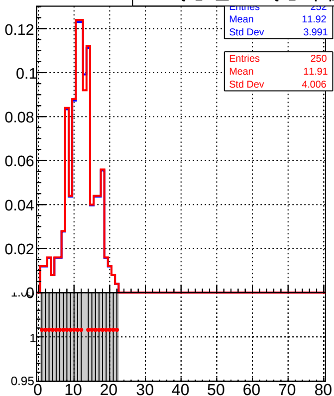
DQM_TT_mkFit-DQM_lowptq_orig DQM_TT_mkFit-DQM_lowptq_mod
