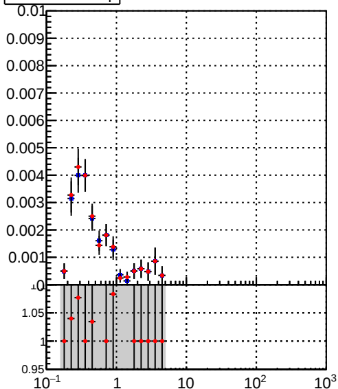
— DQM_TT_mkFit-DQM_lowptq_orig — DQM_TT_mkFit-DQM_lowptq_mod
