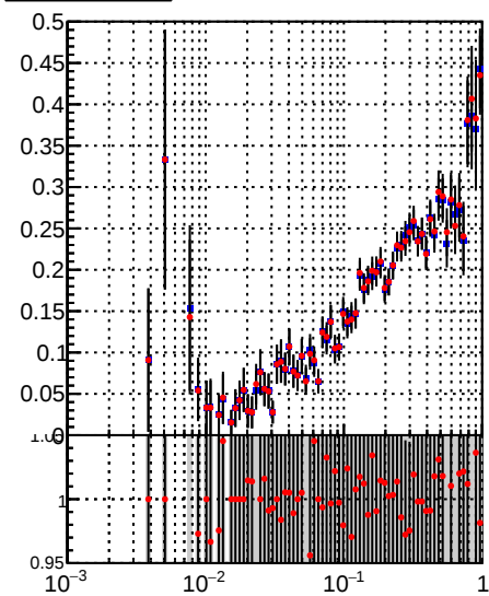
Fake rate vs dr Legend: DQM_TT_mkFit-DQM_lowptq_orig (blue line with circles) DQM_TT_mkFit-DQM_lowptq_mod (red line with circles)
